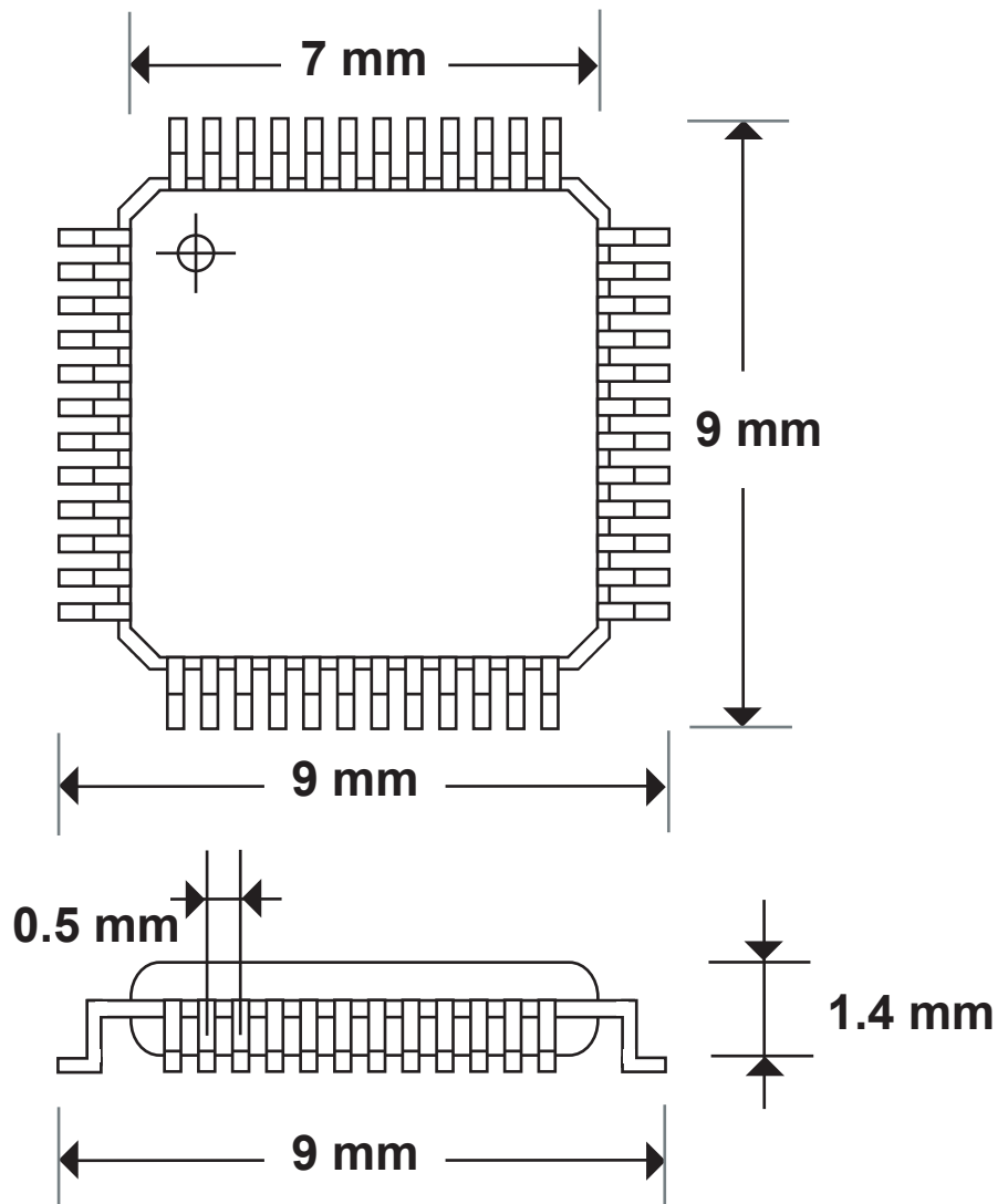
RS232/PS2 chip
